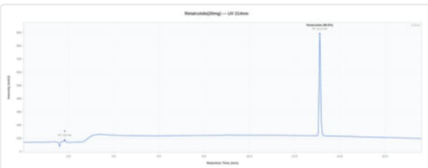
HPLC Chromatogram
