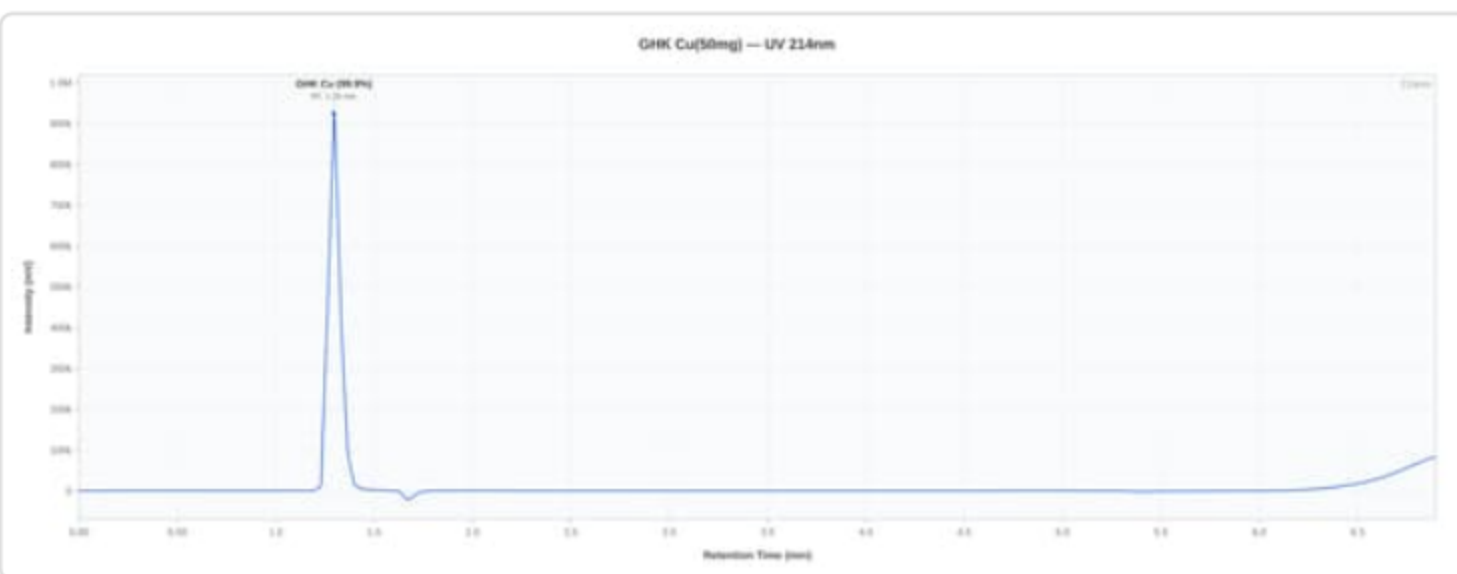
HPLC Chromatogram
