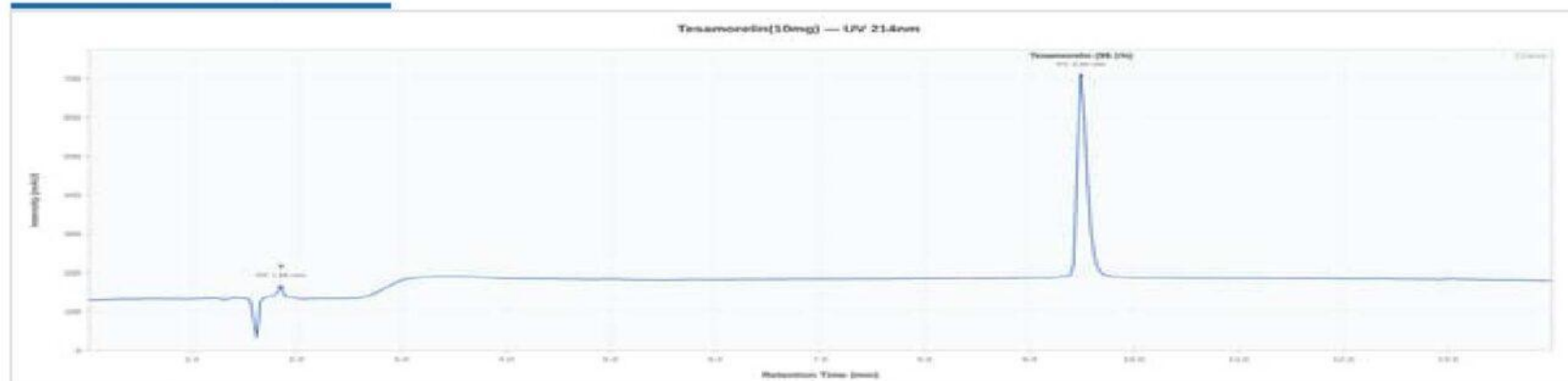
Tesa 10mg - TSM10-06022026: UV Chromatogram
