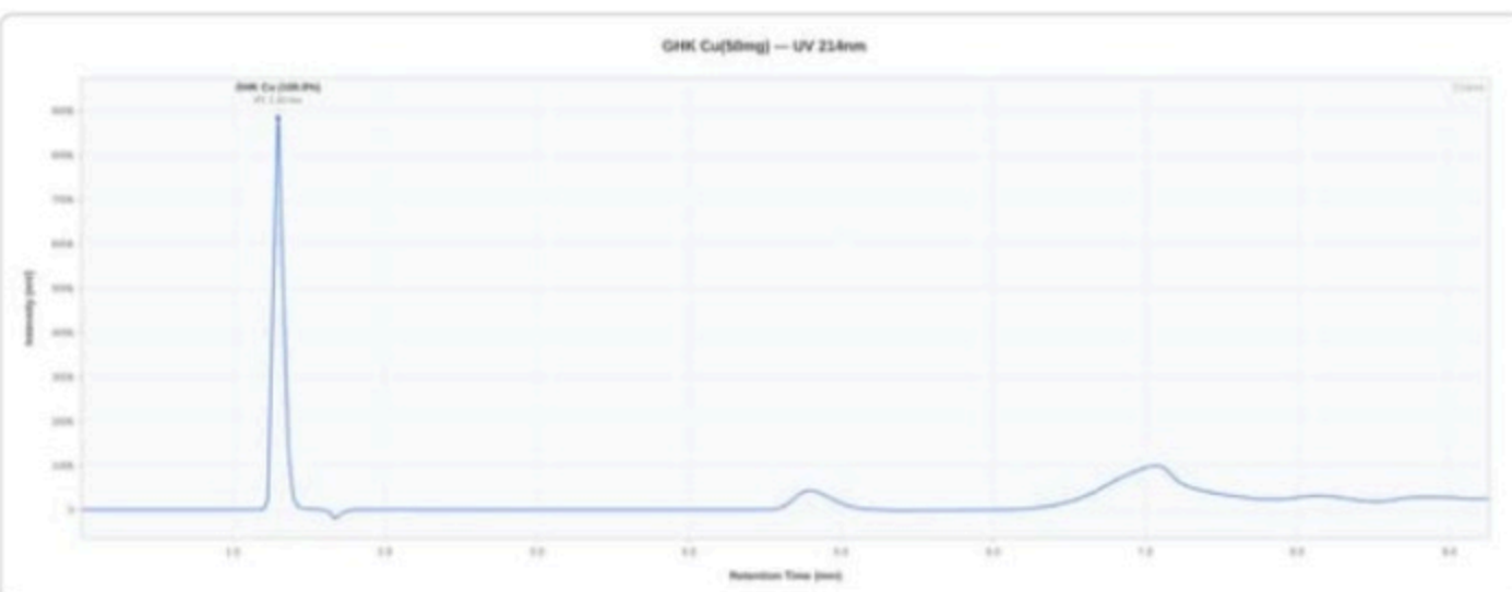
HPLC Chromatogram
