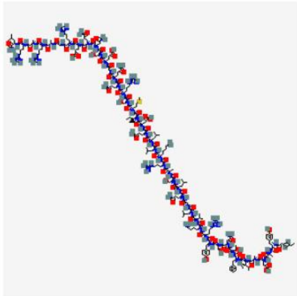
MOLECULAR STRUCTURE
